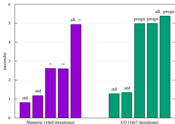
Figure 5: Benchmarks
