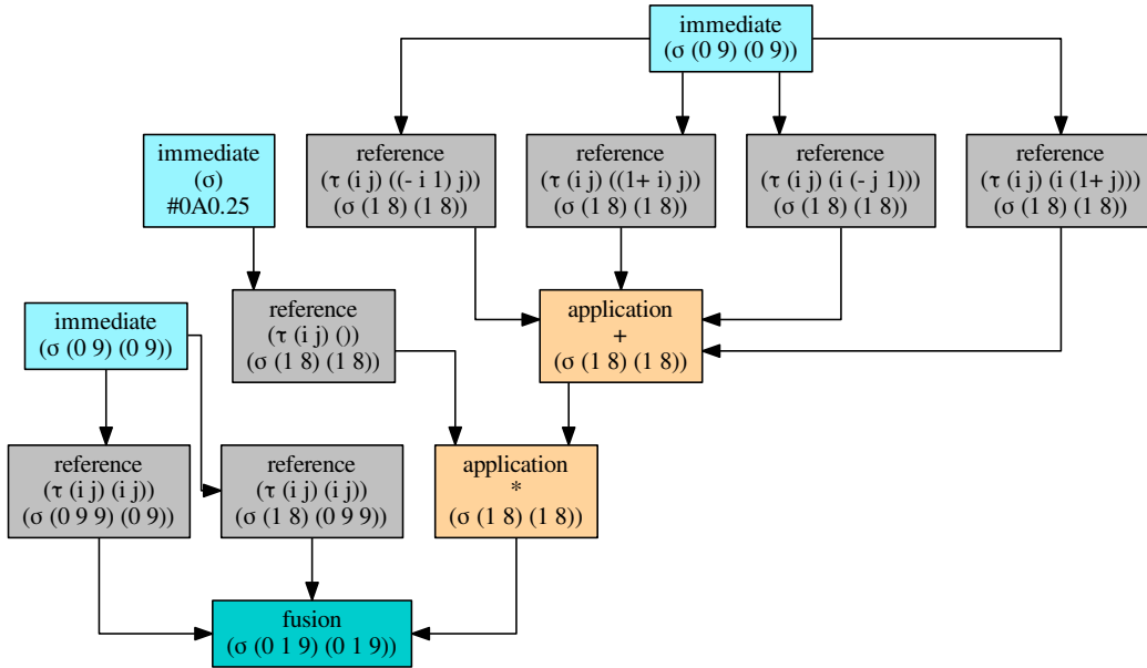
Figure 9: The data flow graph of a single Jacobi iteration on a 10x10 grid.
