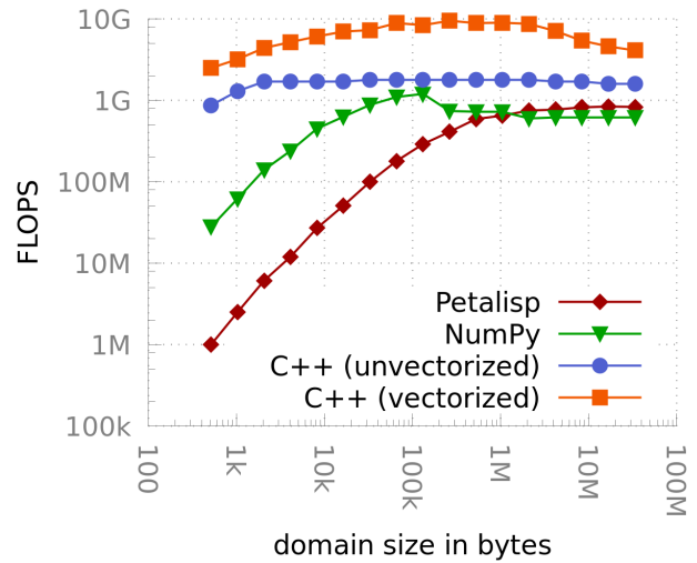
Figure 13: Single-threaded floating point operations per second for Jacobi’s method on a square domain.
